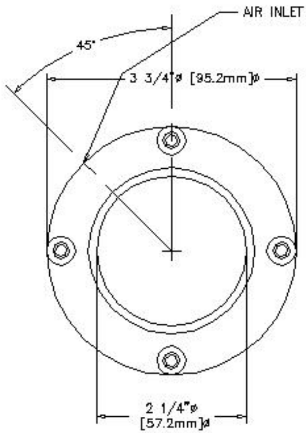
END VIEW
