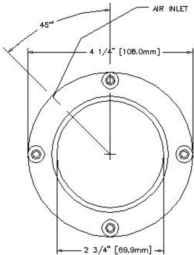
END VIEW
