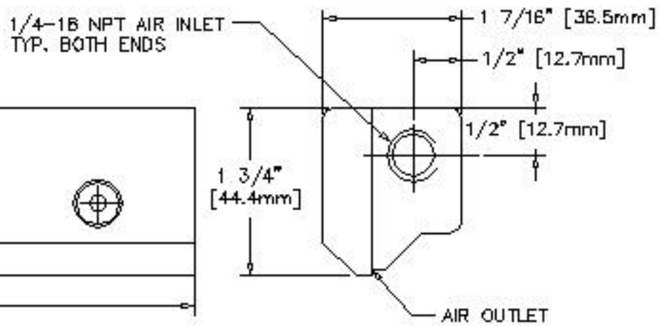
END VIEW
