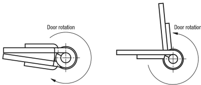
Hinges with closing spring
