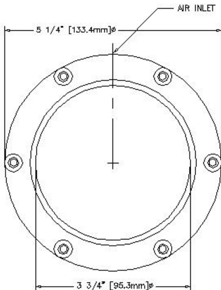
END VIEW
