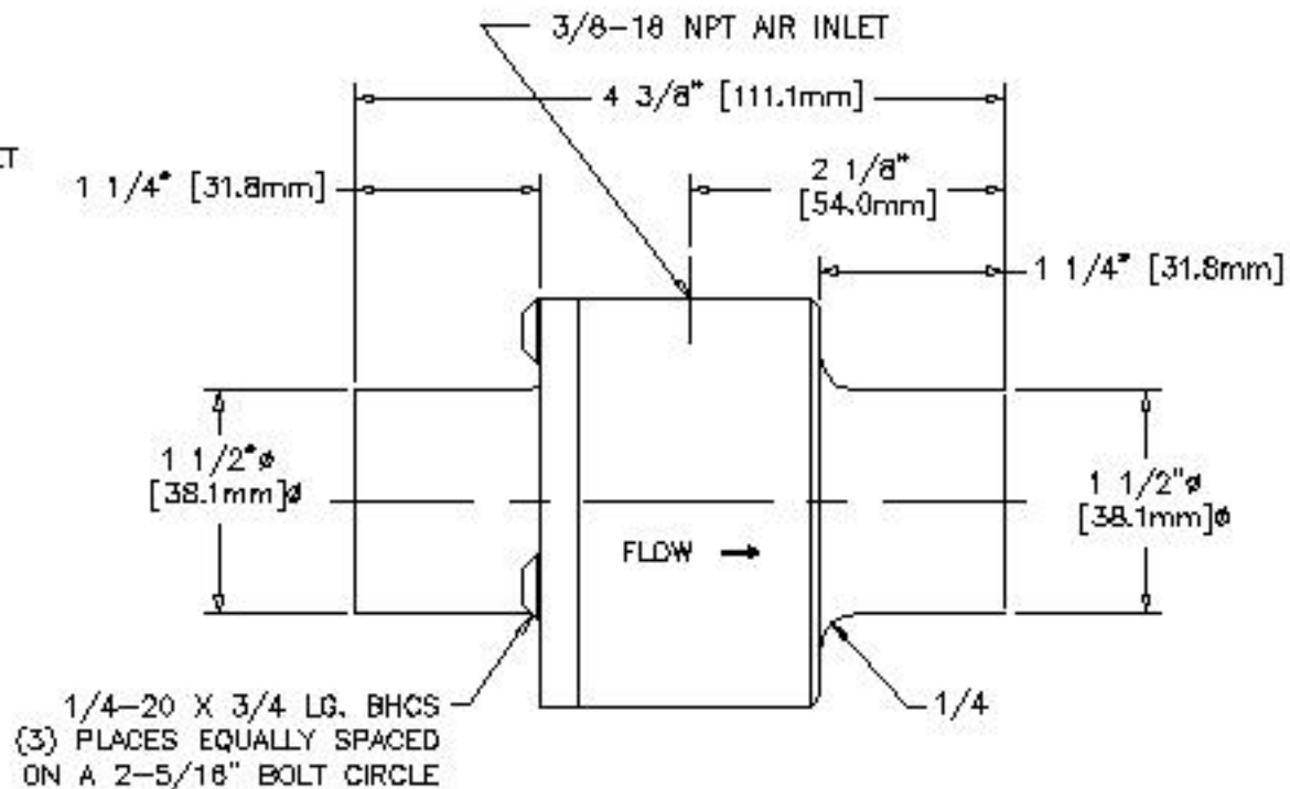
SIDE VIEW
